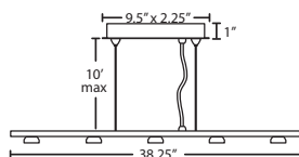
5LP 5 LIGHT LINEAR FIXTURE:
