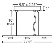
3LP 3 LIGHT LINEAR FIXTURE:
