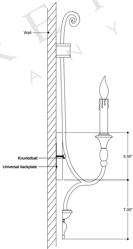
SIDE VIEW
