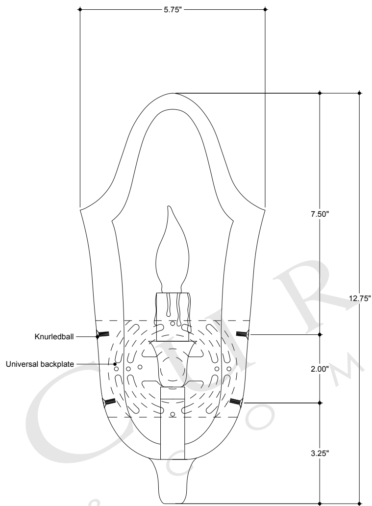
FRONT VIEW
