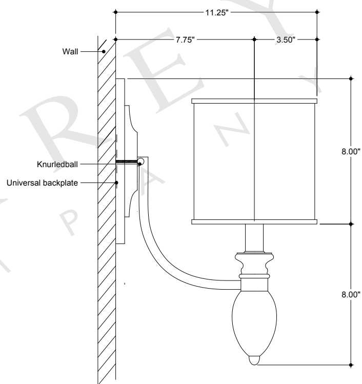
SIDE VIEW
