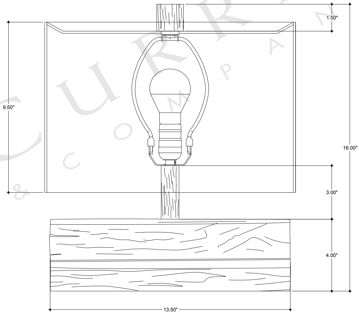
FRONT VIEW
