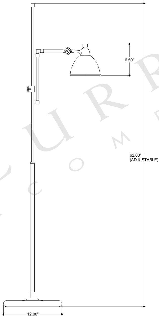
SIDE VIEW
