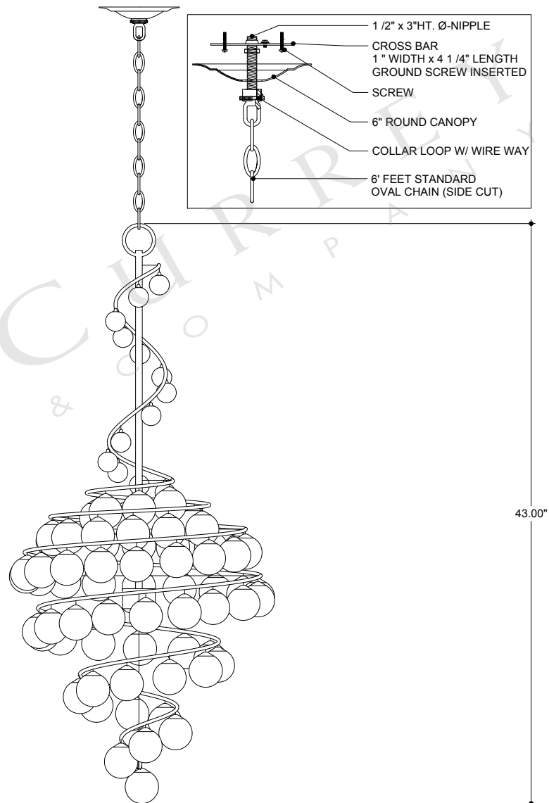
FRONT VIEW
