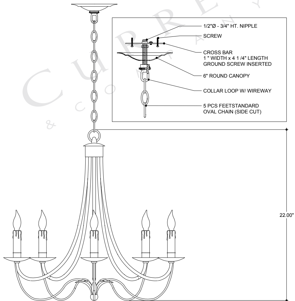
FRONT VIEW
