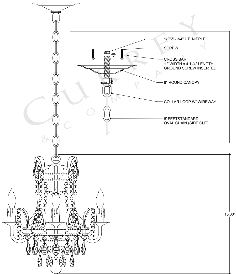
FRONT VIEW
