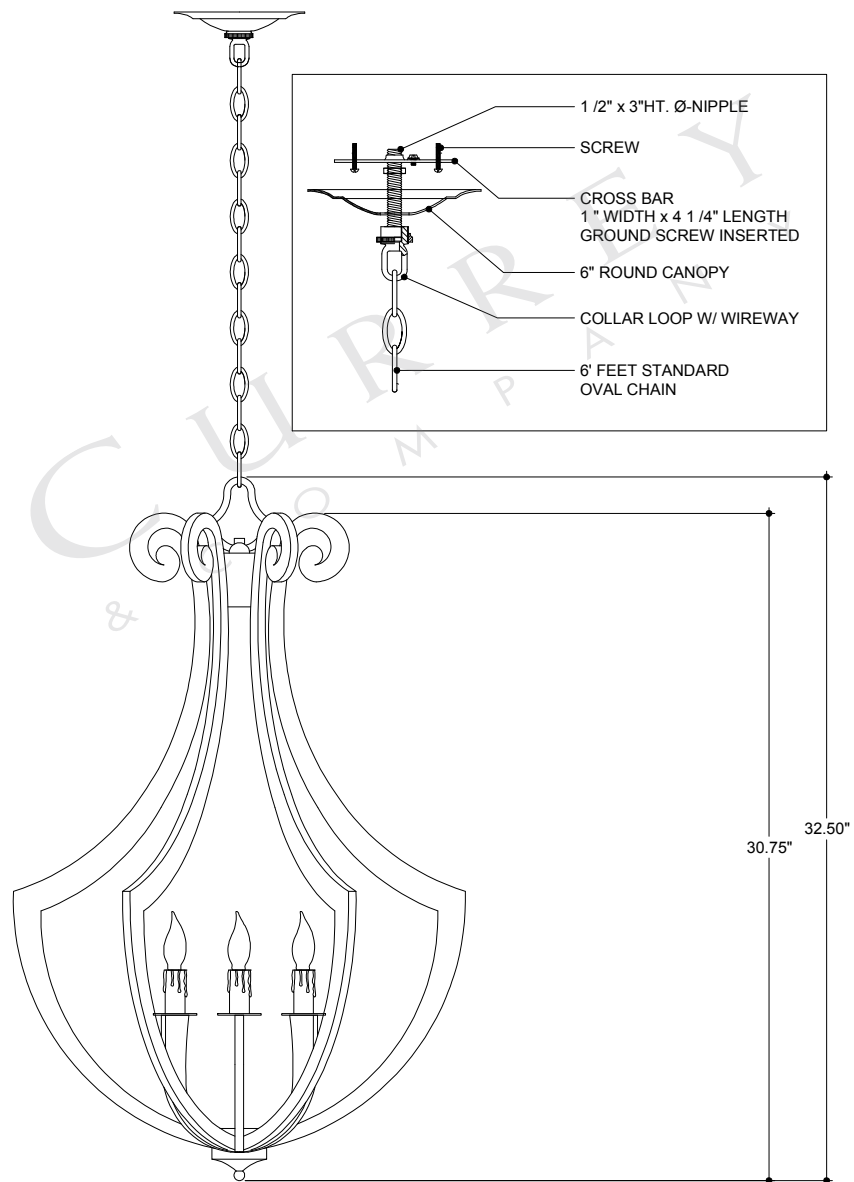
FRONT VIEW
