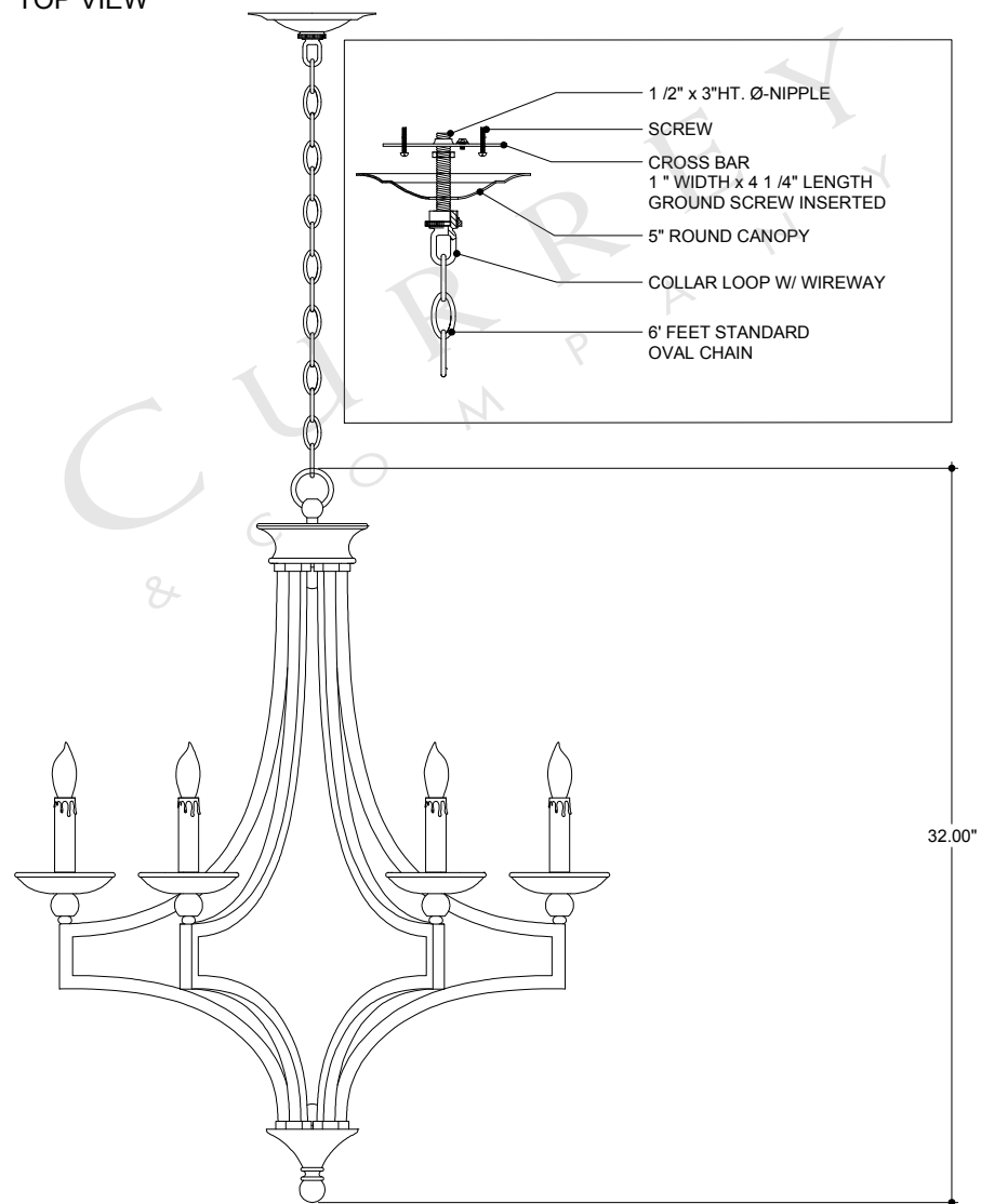
FRONT VIEW
