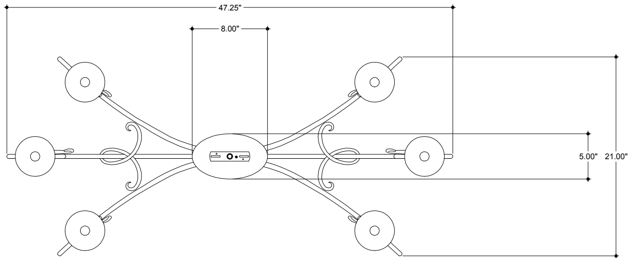
TOP VIEW
