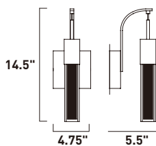
E22760-89PC 1-Light Wall Mount Finish: Polished Chrome Glass: Etched/Bubble 1 x 7.5w LED (Included) | 246 Lumens HCO: 7"
