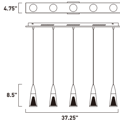
E22477-75PC 5-Light LED Pendant Finish: Polished Chrome Glass: Clear Acrylic 5 x 3W LED (Included) | 1,200 Lumens 11" / 129.75" OAH
