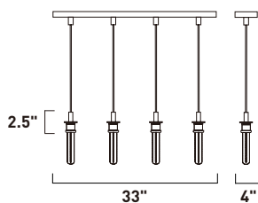
ES93004-BZ Bronze ES93004-SN Satin Nickel 4-Light Pendant Frame 4 x 13W G24q-1 Quad T4 CFL Bulbs 3,120 Lumens 24" / 60" OAH
