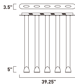
E22355-PC 5-Light LED Pendant Finish: Polished Chrome 5 x 3.5W LED (Included) | 1,225 Lumens 8" / 128" OAH
