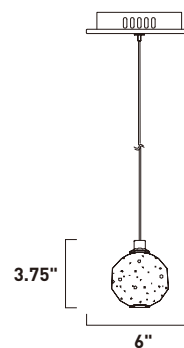
E24500-91PC 1-Light Pendant Finish: Polished Chrome 1 x 1.5W LED (Included) | 105 Lumens 134" OAH
