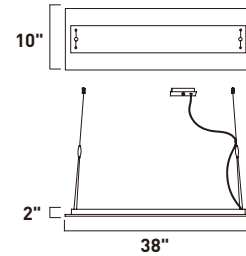
E22123-24AL 2-Light Pendant Finish: Brushed Aluminum (AL) Glass: Clear/White 2 x 21W Mini Bi Pin T5 Bulb (Incl.) | 2,000 Lumens 24" / 90" OAH
