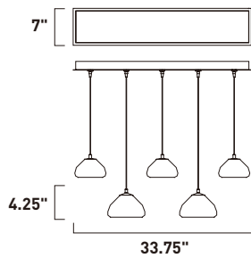
E22524-81PC 5-Light Pendant Finish: Polished Chrome 5 x 2.4W LED (Included) | 2,100 Lumens 7" / 126.5" OAH
