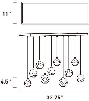
E24487-PC 10-Light Pendant Finish: Polished Chrome 10 x 2.4W LED (Included) | 1,960 Lumens 7" / 126.5" OAH
