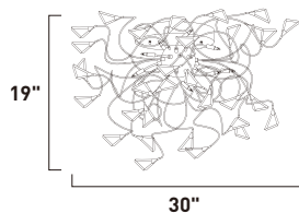
E23261-138PC 12-Light Flush Mount Finish: Polished Chrome Glass: Smoke & Clear 12 x 10W G4 Bulbs (Included) | 1,440 Lumens
