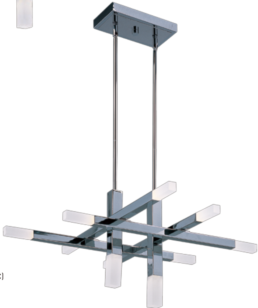
E22514-90PC 10-Light LED Pendant Finish: Polished Chrome Glass: Frost Acrylic 10 x 1.5W LED (Included) | 1,200 Lumens 16" / 58" OAH
