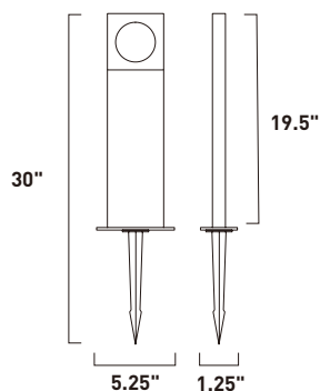
E41369-BZ, SA 1-Light LED Finish: See Images 1 x 9.8W LED (Included) | 480 Lumens
