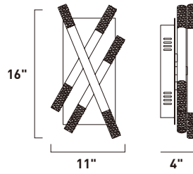
E22480-01PC 6-Light LED Wall Mount Finish: Polished Chrome Glass: Frost Acrylic 6 x 1.5W LED (Included) | 720 Lumens HCO: 2.25"
