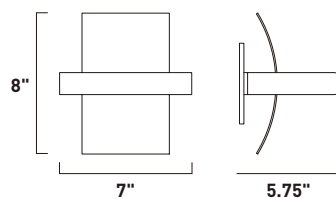
E41312-WT 1-Light LED Wall Mount Finish: White 1 x 6W LED (Included) | 180 Lumens HCO: 3.75"
