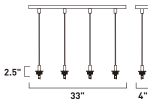
ES92004-BZ Bronze ES92004-SN Satin Nickel 4-Light Pendant Frame 4 x 100W MB Bulbs | 4,600 Lumens 24" / 60" OAH
