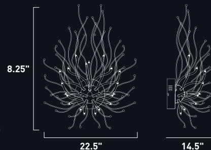
E24472-PC 20-Light LED Wall Mount Finish: Polished Chrome 20 x 0.12W LED Bulbs (Included) | 156 Lumens HCO: 18"
