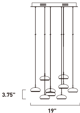
E22558-PC 9-Light LED Pendant Finish: Polished Chrome Frosted Acrylic Lens 9 x 4.8W LED (Integrated) | 2,592 Lumens 6" / 120" OAH
