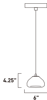
E22521-81PC 1-Light Pendant Finish: Polished Chrome 1 x 2.4W LED (Included) | 196 Lumens 134" OAH
