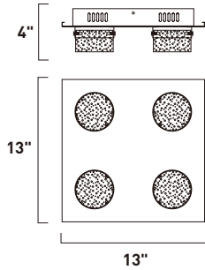
E22772-91PC 4-Light Flush Mount Finish: Polished Chrome Glass : Bubble Crystal 4 x 7.5W LED (Included) | 1,932 Lumens
