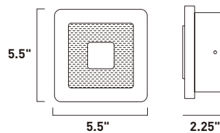
E41316-90SA 4-Light LED Wall Mount Finish: Satin Aluminum Glass: Frosted 4 x 1W LED (Included) | 320 Lumens HCO: 2.75"
