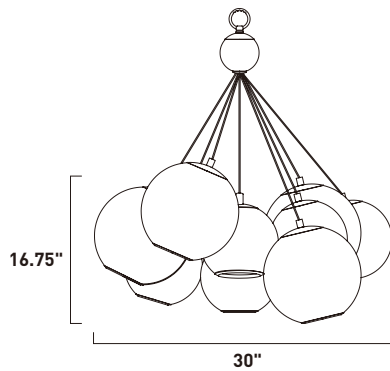
E22787-81PC 9-Light LED Pendant Finish: Polished Chrome Glass: Mirror Chrome 5 x 1.5W + 4 x 4.5W LED (Included) | 2,040 Lumens 40.5" / 115" OAH
