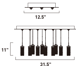
E95488-148PC 10-Light Pendant Finish: Polished Chrome 10 x 7.5W LED (Included) | 5,250 Lumens 134" OAH
