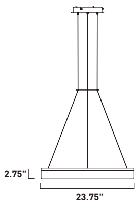
E22453-11MS LED Pendant Finish: Metallic Silver Glass: Frost Acrylic 24W LED (Included) | 1,680 Lumens 35.75" / 51.5" OAH
