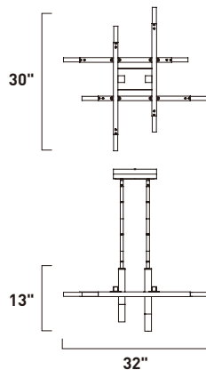
E22514-90PC 10-Light LED Pendant Finish: Polished Chrome Glass: Frost Acrylic 10 x 1.5W LED (Included) | 1,200 Lumens 16" / 58" OAH
