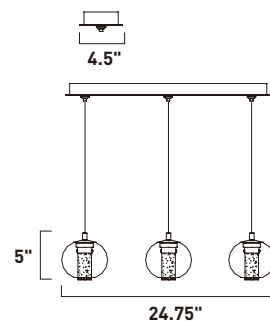
E22564-81PC 3-Light Pendant Finish: Polished Chrome Glass : Clear 3 x 3W LED (Included) | 450 Lumens 134" OAH
