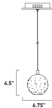
E24480-PC 1-Light Pendant Finish: Polished Chrome 1 x 2.4W LED (Included) | 196 Lumens 134" OAH
