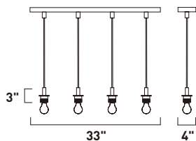
ES92004-BZ Bronze ES92004-SN Satin Nickel 4-Light Pendant Frame 4 x 100W MB Bulbs | 4,600 Lumens 24" / 60" OAH
