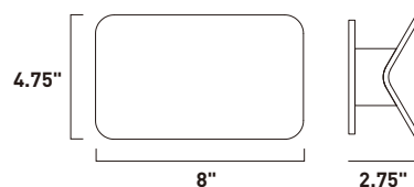
E41309-SA 2-Light LED Wall Mount Finish: Satin Aluminum 2 x 2.7W LED Bulbs (Included) | 600 Lumens HCO: 2.5"
