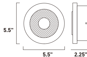
E41315-90SA 3-Light LED Wall Mount Finish: Satin Aluminum Glass: Frosted 3 x 1W LED (Included) | 240 Lumens HCO: 2.75"
