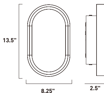
E22440-11MS LED Wall Mount Finish: Metallic Silver Glass: Acrylic 25W LED (Included) | 1,500 Lumens HCO: 6.75"
