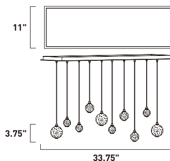
E24507-91PC 10-Light Pendant Finish: Polished Chrome 10 x 1.5W LED (Included) | 1,050 Lumens 6" / 126" OAH
