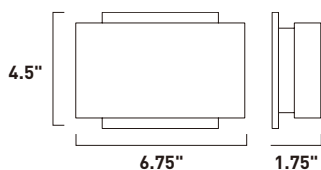
E41310-SA 6-Light LED Wall Mount Finish: Satin Aluminum 6 x 1.8W LED (Included) | 560 Lumens HCO: 2.25"
