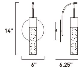
E22770-91PC 1-Light Wall Mount Finish: Polished Chrome Glass : Bubble Crystal 1 x 7.5W LED (Included) | 246 Lumens HCO:7"
