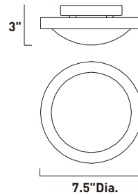
E53831-09SN 1-Light LED Flush/Wall Mount Finish: Satin Nickel (SN) Glass: Frosted White 1 x 5W LED (Included) | 370 Lumens HCO: 3.75"
