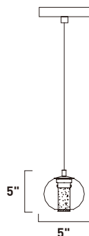
E22561-81PC 1-Light Pendant Finish: Polished Chrome Glass : Clear 1 x 3W LED (Included) | 150 Lumens 134" OAH
