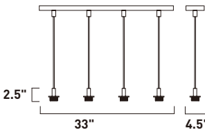
ES93004-BZ Bronze ES93004-SN Satin Nickel 4-Light Pendant Frame 4 x 13W G24q-1 Quad T4 CFL Bulbs 3,120 Lumens 24" / 60" OAH
