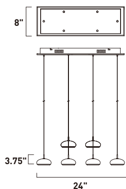
E22556-PC 6-Light LED Pendant Finish: Polished Chrome Frosted Acrylic Lens 6 x 4.8W LED (Integrated) | 1,728 Lumens 6" / 120" OAH
