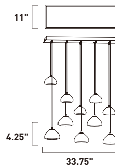
E22528-81PC 10-Light Pendant Finish: Polished Chrome 10 x 2.4W LED (Included) | 4,200 Lumens 7" / 126.5" OAH
