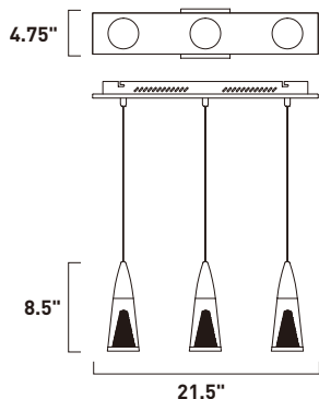
E22476-75PC 3-Light LED Pendant Finish: Polished Chrome Glass: Clear Acrylic 3 x 3W LED (Included) | 720 Lumens 11" / 129.75" OAH
