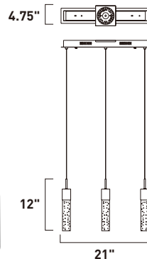
E22773-91PC 3-Light Pendant Finish: Polished Chrome Glass : Bubble Crystal 3 x 7.5W LED (Included) | 738 Lumens 14" / 59" OAH
