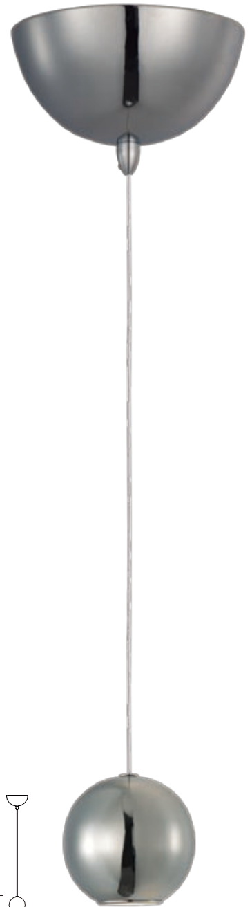
E22191-PC 1-Light LED Pendant Finish: Polished Chrome 1 x 3W LED (Included) / 360 Lumens 6" / 128" OAH
