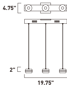
E22493-11PC 3-Light LED Pendant Finish: Polished Chrome Glass: Frost Acrylic 3 x 4W COB LED (Included) | 777 Lumens 5" / 125" OAH
