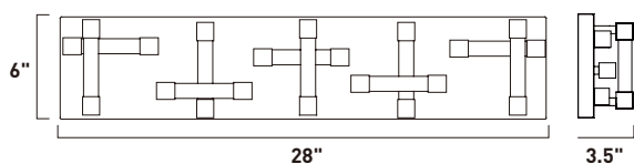
E22518-90PC 20-Light LED Bath Vanity Finish: Polished Chrome Glass: Frost Acrylic 20 x 1.5W LED (Included) | 2,400 Lumens HCO: 3"
