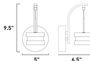
E22280-01PC 1-Light LED Wall Mount E22680-01PC (Dimmable Version) Finish: Polished Chrome Glass: White 1 x 4.8W LED Bulb (Included) | 288 Lumens HCO: 6.75"
