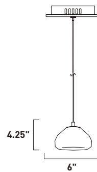
E22520-81PC 1-Light Pendant Finish: Polished Chrome 1 x 2.4W LED (Included) | 196 Lumens 134" OAH
