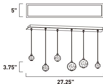
E24505-91PC 6-Light Pendant Finish: Polished Chrome 6 x 1.5W LED (Included) | 630 Lumens 6" / 126" OAH
