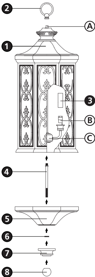
Drawing 1 - Fixture Assembly
