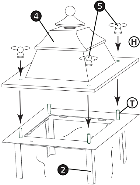
Drawing 3 - Fixture Mounting
