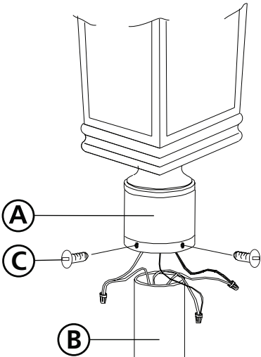
Drawing 3 - Fixture Mounting
