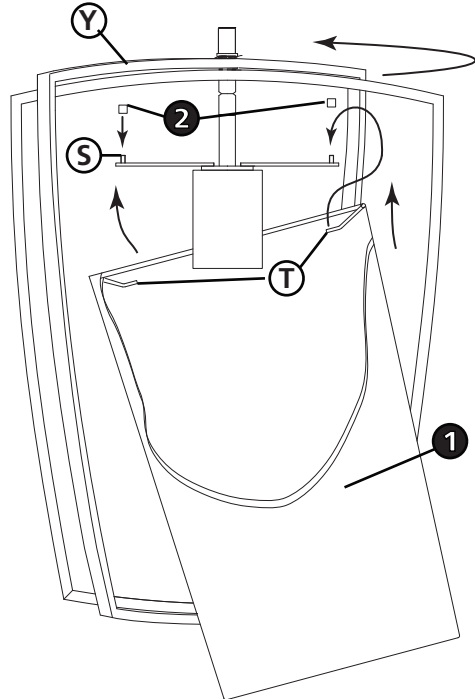
Drawing 1 - Shade Installation
