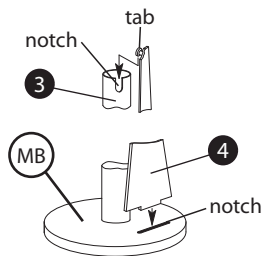
Drawing - 3 Rod installation
