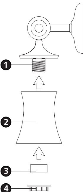
Drawing 2 - Fixture Assembly
