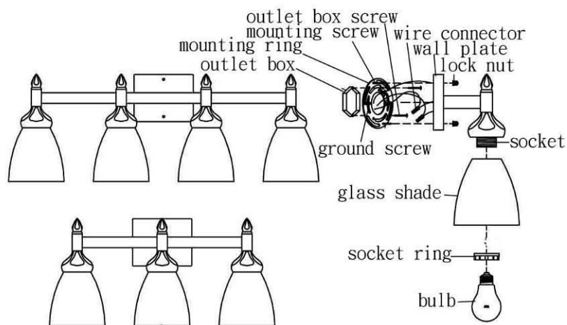
Fig.1: Install for downwards
