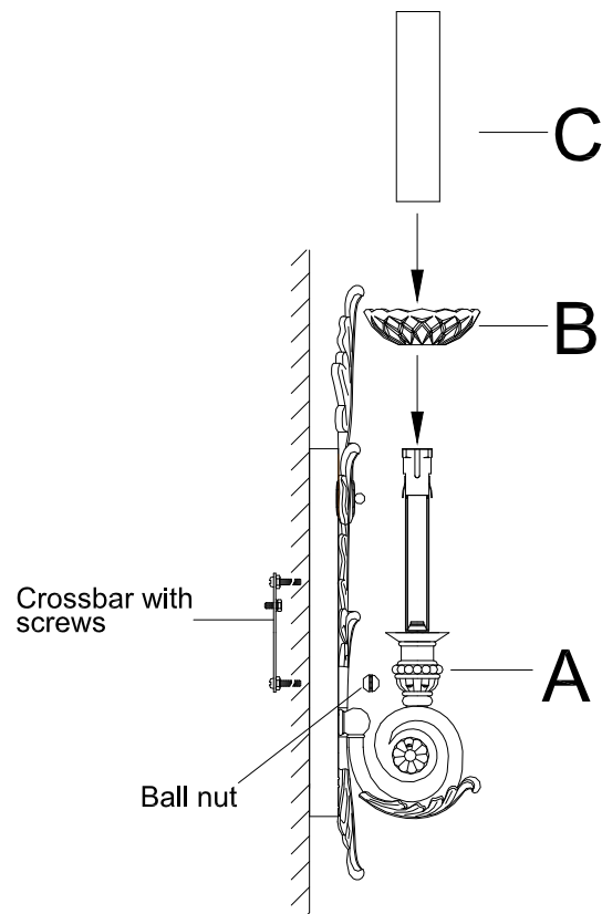
Side view of fixture
