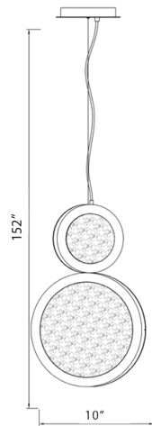
HF5011-PN Polished Nickel 16"H x 10"L x 2"W 152" OAH 32W/120V LED 2360lm 3500K Dimmable
