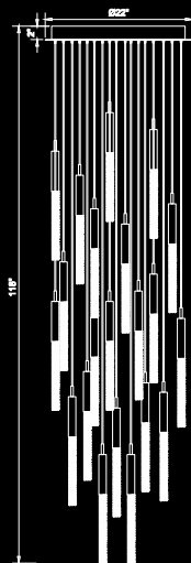
HF2021-FR-PN Polished Nickel 22"W x 118" OAH (21) G-9 Base Sockets 74W / 120V 6300 Lumens 3000K
