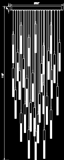
HF2031-BOA-PN Polished Nickel 30"W x 118" OAH (31) G-9 Base Sockets 109W / 120V 9300 Lumens 3000K
