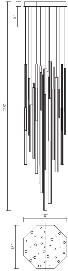
HF7018-BB Brushed Brass 18"W x 216"H 216" OAH (18) G-9 Base Sockets 63W / 120V 5400 Lumens 3000K
