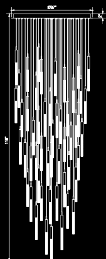
HF2051-BOA-PN Polished Nickel 37"W x 118" OAH (51) G-9 Base Sockets 178.5W / 120V 15300 Lumens 3000K
