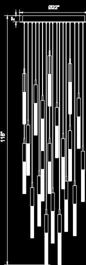
HF2021-BOA-PN Polished Nickel 22"W x 118" OAH (21) G-9 Base Sockets 74W / 120V 6300 Lumens 3000K
