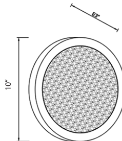
HF5012-PB Polished Brass Wall or Ceiling Mount 10"D x 3"EXT 20.5W/120V LED 1500lm 3500K Dimmable
