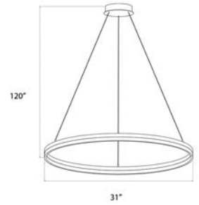
HF5028-GL Brushed Gold 31"W x 1.5"H 35W / 120V 1700 Lumens 3000K
