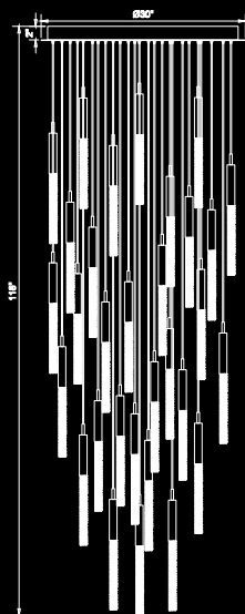
HF2031-FR-PN Polished Nickel 30"W x 118" OAH (31) G-9 Base Sockets 109W / 120V 9300 Lumens 3000K
