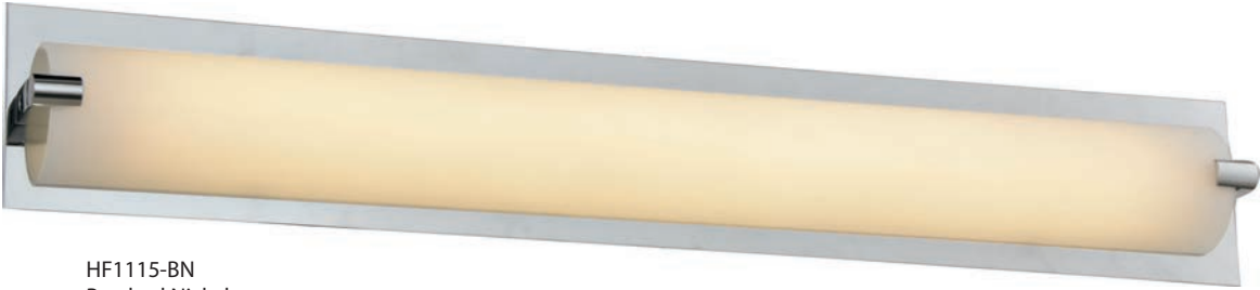
HF1116-BN Brushed Nickel 38"L x 2"EXT x 4"H 45W/120V LED 3600lm 3000K Dimmable
