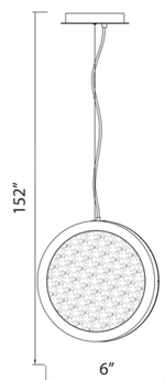
HF5014-PB Polished Brass 6"D x 2"W 152" OAH 11.5W/120V LED 860lm 3500K Dimmable
