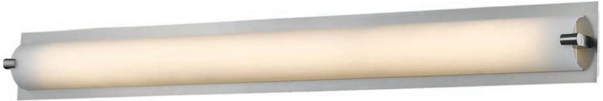
HF1115-CH Polished Chrome 26"L x 2"EXT x 4"H 30W/120V LED 2400lm 3000K Dimmable
