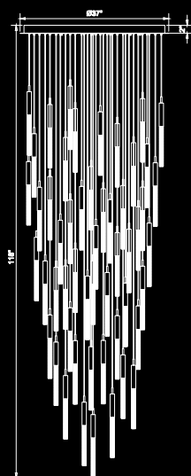
HF2051-BOA-BB Brushed Brass 37"W x 118" OAH (51) G-9 Base Sockets 178.5W / 120V 15300 Lumens 3000K
