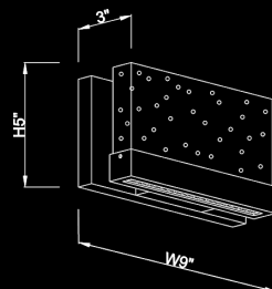
HF3001-PN 9"W x 5"H x 3"EXT 8W/120V LED 800lm 3000K Dimmable
