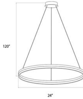
HF5027-BK Black 24"W x 1.5"H 28W / 120V 1050 Lumens 3000K
