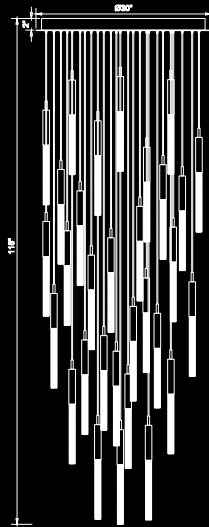
HF2031-BOA-BB Brushed Brass 30"W x 118" OAH (31) G-9 Base Sockets 109W / 120V 9300 Lumens 3000K
