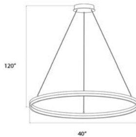
HF5029-BK Black 40"W x 2"H 66W / 120V 1700 Lumens 3000K
