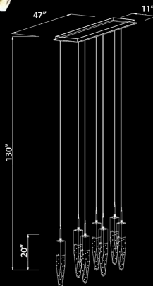
HF1900-7-AP-CH Polished Chrome 11"W x 46.5"H x 130" OAH (7) GU-10 Base LED 42W Total / 120V 2800 Lumens 3000K
