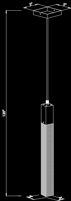
HF1901-01-BOA-DBZ Dark Bronze 5" Square Canopy 2" W x 24" H 120" OAH (1) GU10 Base LED 6W 120V 3000k 400 Lumens Dimmable Bulb Included
