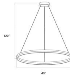
HF5029-GL Brushed Gold 40"W x 2"H 66W / 120V 1700 Lumens 3000K
