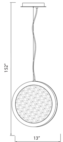
HF5020-PN Polished Nickel 13"D x 2"W 152" OAH 26.5W/120V LED 2000lm 3500K Dimmable
