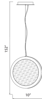
HF5018-PN Polished Nickel 10"D x 2"W 152" OAH 20.5W/120V LED 1500lm 3500K Dimmable
