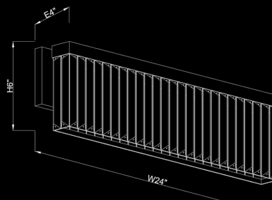
HF4002-PN 24"W x 6"H x 4"EXT 30 Watt 120 Volt 2400 Lumens 3000K
