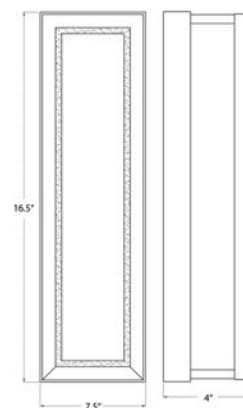
HF9404-BLK Black 16.5"H x 7.5"W x 4" Ext OAH 16.5" 17 Watt / 12V 3000K / 90 CRI 550 Lumens
