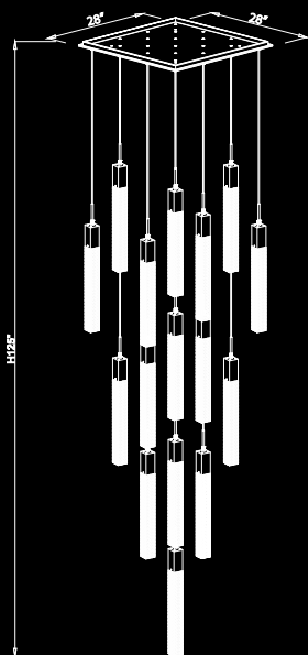
HF1905-13-BOA-BB Brushed Brass 20"W x 104"H (13) GU10 Base LED 6W 120V 3000k 5200 Lumens Dimmable Bulbs Included
