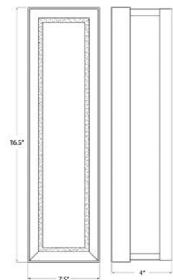
HF9404-GLD Gold 16.5"H x 7.5"W x 4" Ext OAH 16.5" 17 Watt / 12V 3000K / 90 CRI 550 Lumens
