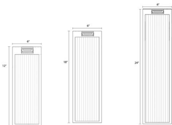
AV9901-SLV Silver 6" W x 12" H x 4" Ext 6W / 120V 290 Lumens 3000K
