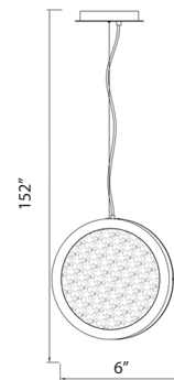
HF5014-PN Polished Nickel 6"D x 2"W 152" OAH 11.5W/120V LED 860lm 3500K Dimmable
