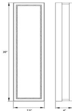
HF9405-GLD Gold 30"H x 7.5"W x 4" Ext 25 Watt / 12V 3000K / 90 CRI 900 Lumens
