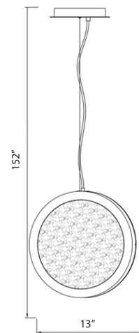
HF5020-PB Polished Brass 13"D x 2"W 152" OAH 26.5W/120V LED 2000lm 3500K Dimmable
