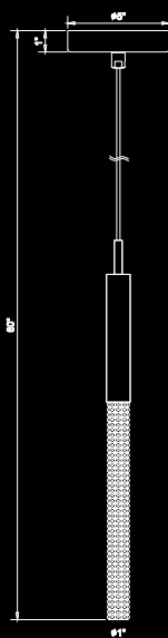
HF2020-BOA-BB Brushed Brass 5"W x 108" OAH (1) G-9 Base Socket 3.5W / 120V 300 Lumens 3000K Pendant Body Height 19"
