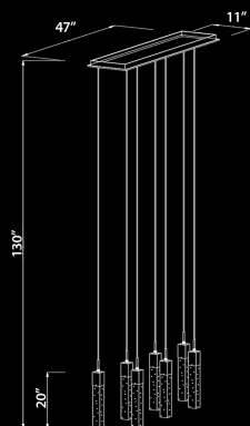
HF1900-7-GL-CH Polished Chrome 11"W x 46.5"H x 130" OAH (7) GU-10 Base LED 42W Total / 120V 2800 Lumens 3000K
