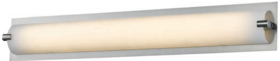
HF1114-CH Polished Chrome 15.5"L x 2"EXT x 4"H 15W/120V LED 1200lm 3000K Dimmable
