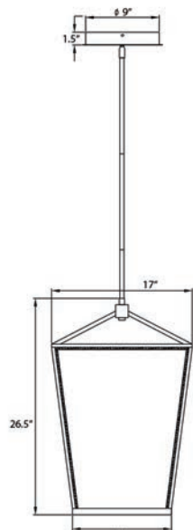
HF9401-GLD Gold 17"W x 26.5"H OAH 70" 64 Watt / 12V 3000K / 90 CRI 3600 Lumens
