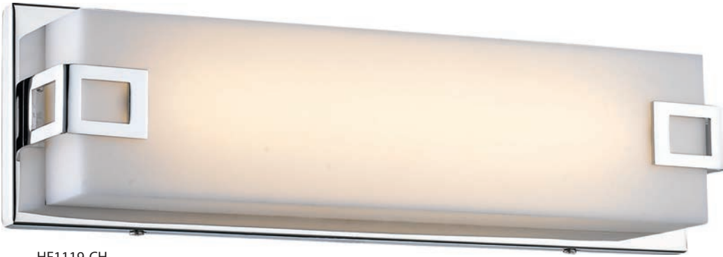
HF1119-CH Polished Chrome 37.5"L x 5.5"EXT x 4"H 45W/120V LED 3600lm 3000K Dimmable
