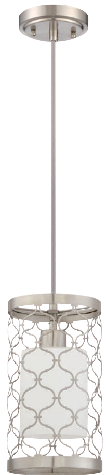
40591-SN - 1 Light Pendant 6.25"W x 11"H; 10' Cord 60 Watt Medium Base; White Frosted Glass - 4.38"D
