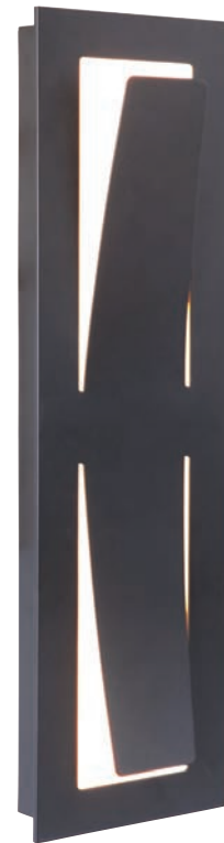
Z4812-MN-LED - Wall Mount 5.25"W x 17.75"H x 2.75"E; 4.5"W x 17"H Backplate Frosted Acrylic Lens; 17 Watt LED, 1890 Lumens
