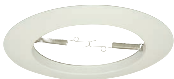
T-501 - Open Ring, PAR 38, BR40/150 Watt Max. 7.75"D; White; Individually Packed
