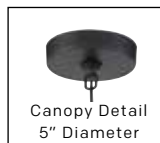
53303-FB - 3 Light Vanity 23.75" W x 10.5" H x 7.25" E 5" Dia x 1" D Backplate 40 Watt Candelabra Base
