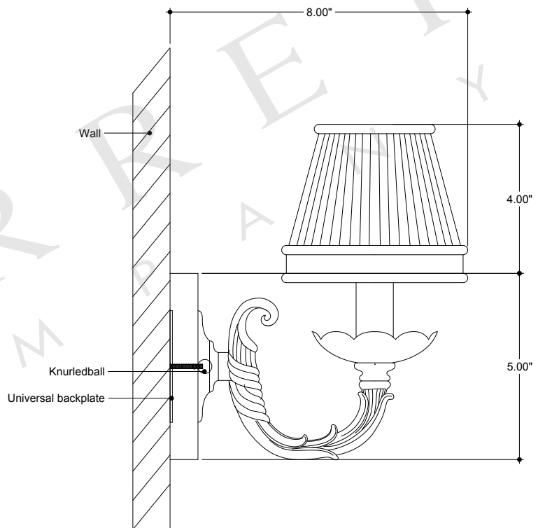
SIDE VIEW
