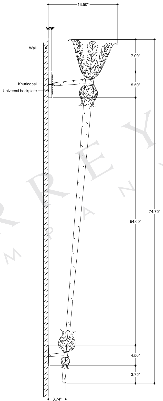
SIDE VIEW
