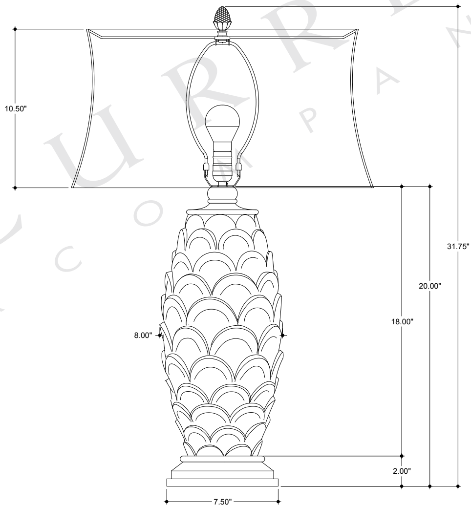
FRONT VIEW
