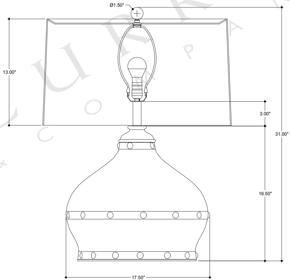
FRONT VIEW
