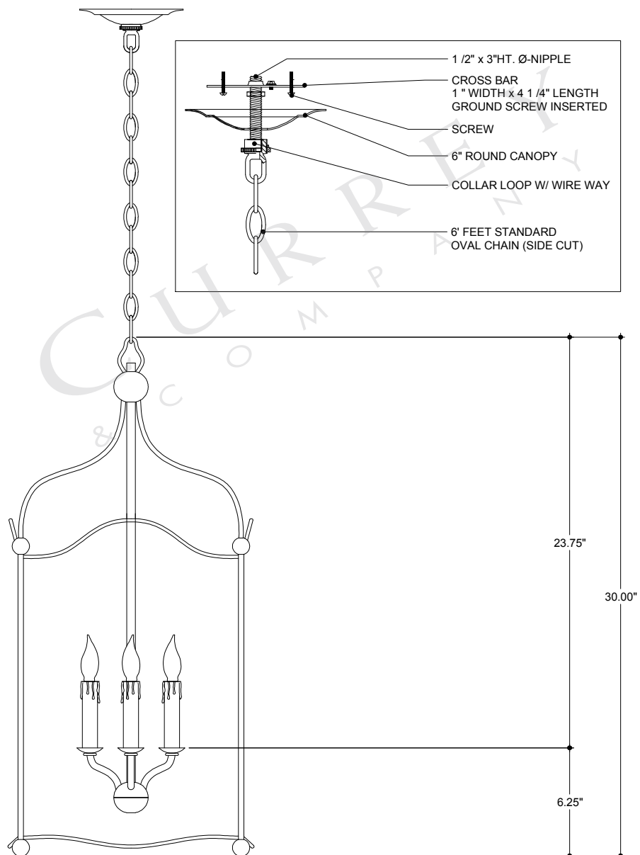
FRONT VIEW
