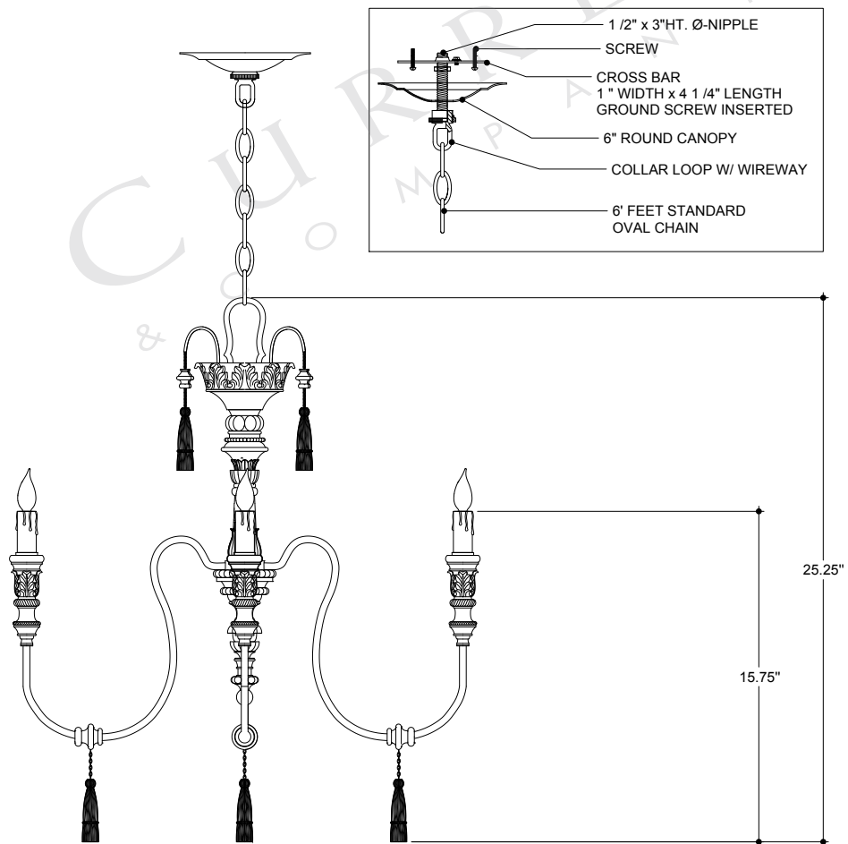
FRONT VIEW
