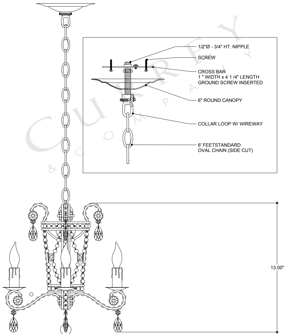
FRONT VIEW
