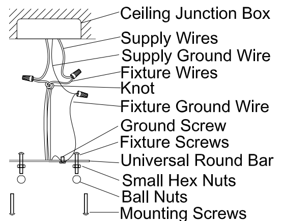
Wiring Drawing ( 2 )
