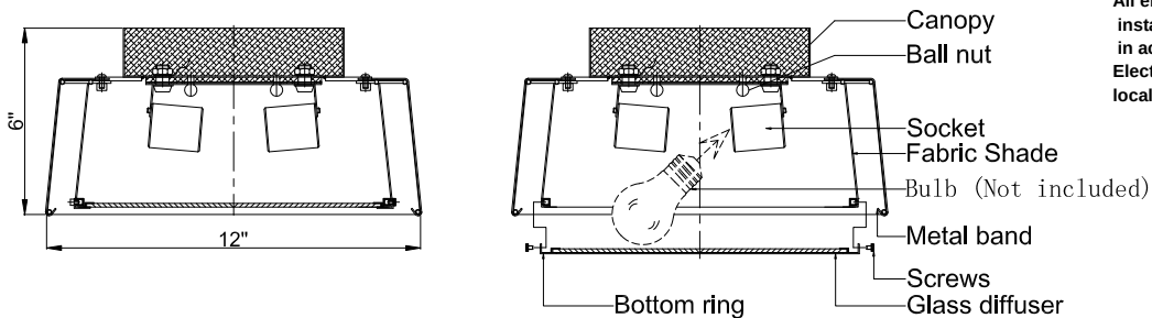
Drawing ( 1 )
