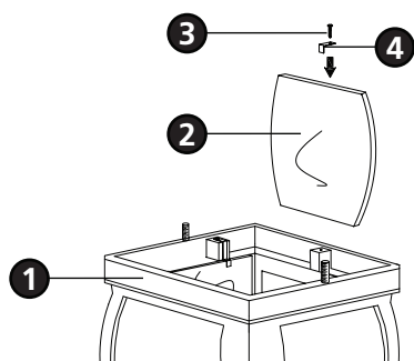
Drawing 1 - Glass Installation
