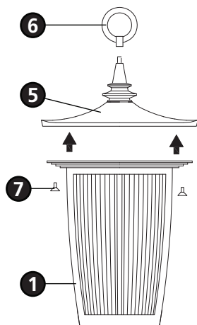
Drawing 2 - Fixture Assembly
