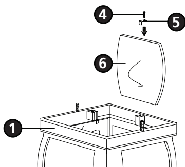
Drawing 4 - Glass Installation
