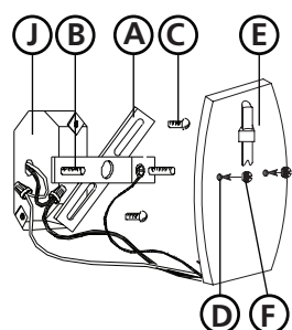
Drawing 3 - Cage Removal
