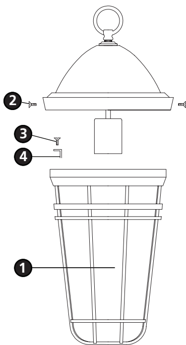
Drawing 1 - Glass Replacement
