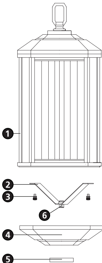
Drawing 1 - Fixture Assembly
