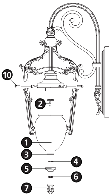
Drawing 4 - Fixture Assembly
