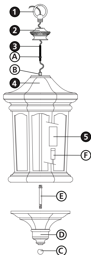
Drawing 1 - Fixture Assembly
