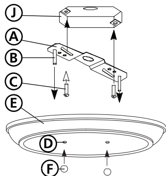
Drawing 3 - Fixture Mounting
