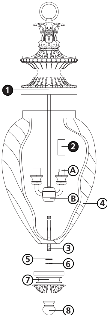
Drawing 1 - Fixture Assembly
