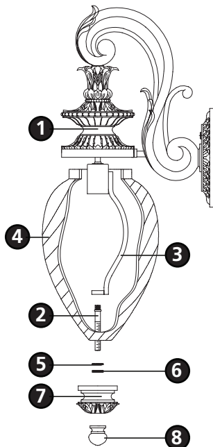
Drawing 3 - Fixture Assembly
