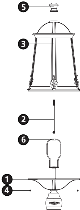
Drawing 1 - Fixture Assembly
