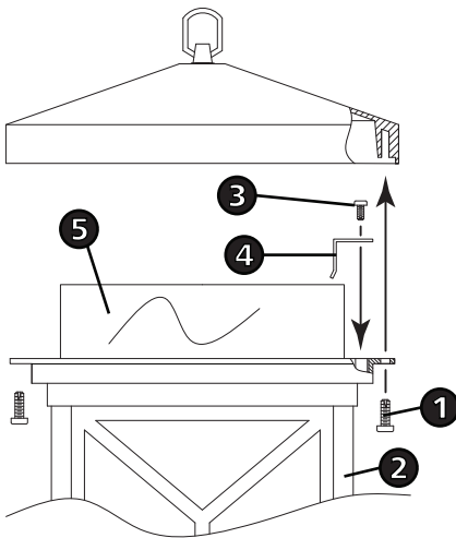
Drawing 1 - Fixture Assembly
