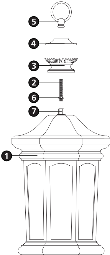
Drawing 1 - Fixture Assembly
