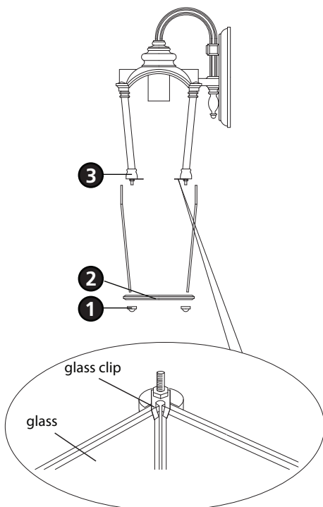
Drawing 3 - Glass Installation
