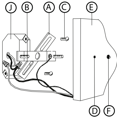
Drawing 3 - Glass Installation
