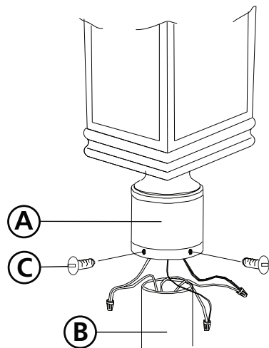
Drawing 4 - Fixture Mounting
