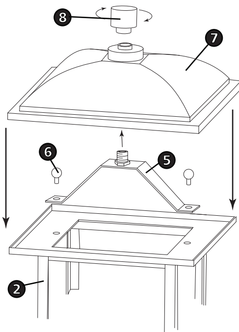
Drawing 4 - Fixture Mounting
