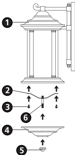
Drawing 3 - Fixture Assembly
