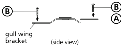
Drawing 1 - Strap Detail
