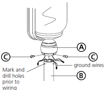
Drawing 3 – Fixture Mounting
