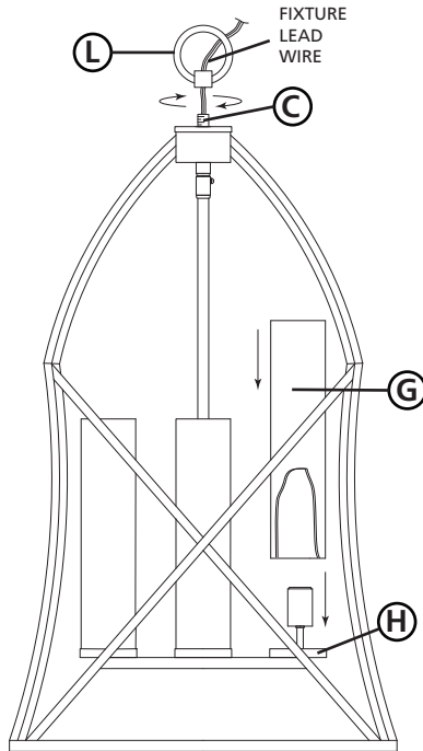
Drawing 1 – Assembly
