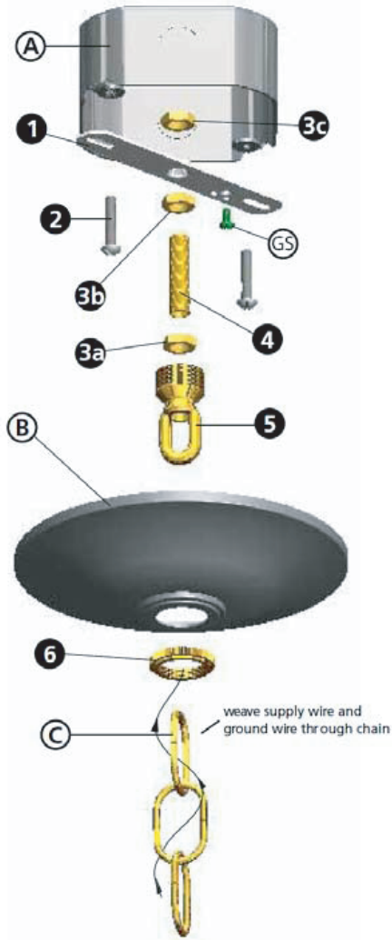
Drawing 2 – Canopy Adjustment
