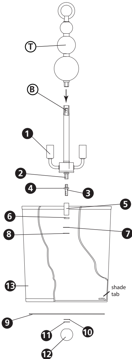
Drawing 1 - Fixture Assembly
