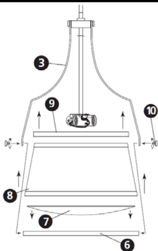
Drawing 3 – Assembly Detail
